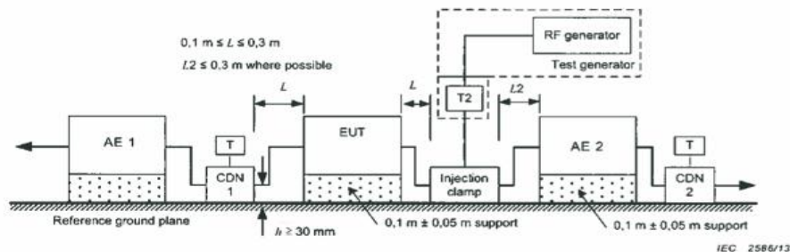
Schematic setup for immunity test used for injection clamp
